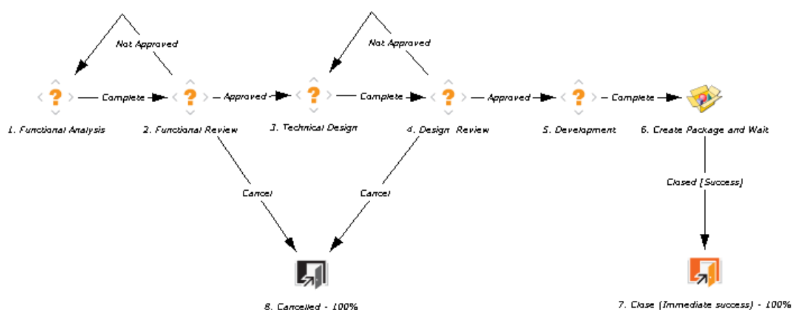
Figure C-5. OraApps Design & Development workflow
